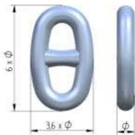
Common Link
