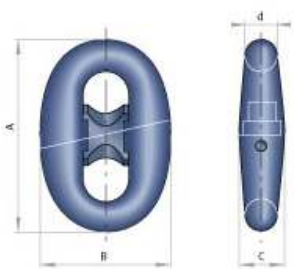
Kenter Shackle
